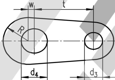
Style - "C" Pin for outer Link
