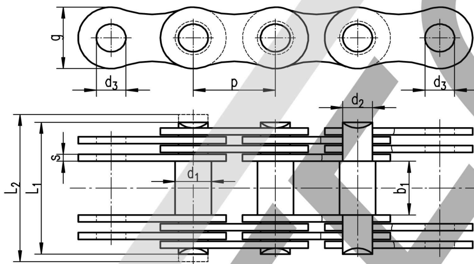
Style - "A" Endlink
